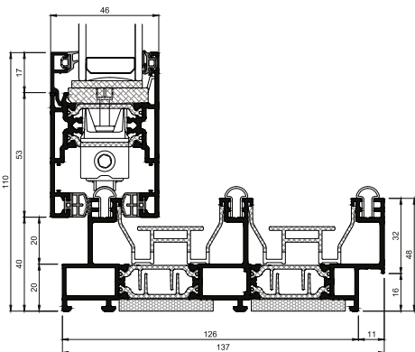
TRIPLE TRACK
