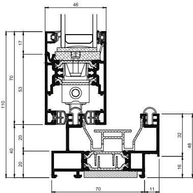
DOUBLE TRACK
