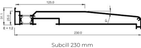
CILLS
