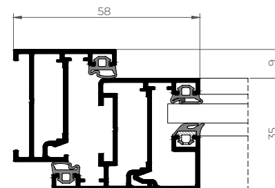
LATERAL SECTION
