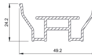
4907 Frame cover
