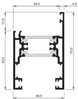
COR-4420 Sash
