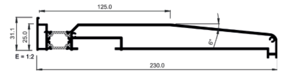
3838 230mm Cill
