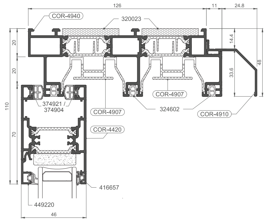
Triple-Track Bottom
