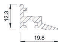
4408 Interlock cover
